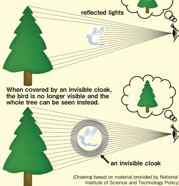
Figure 2 Theory of invisible cloaks
