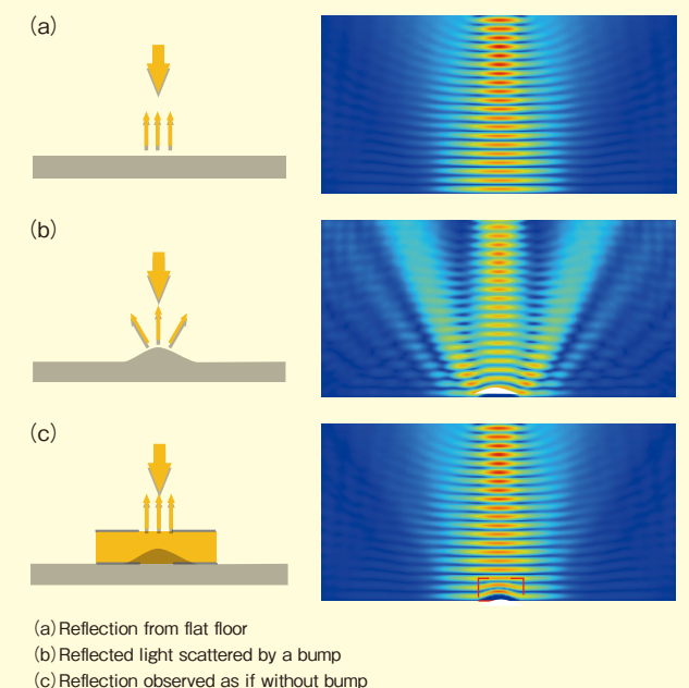
Figure 3 Theory of illusion carpets
